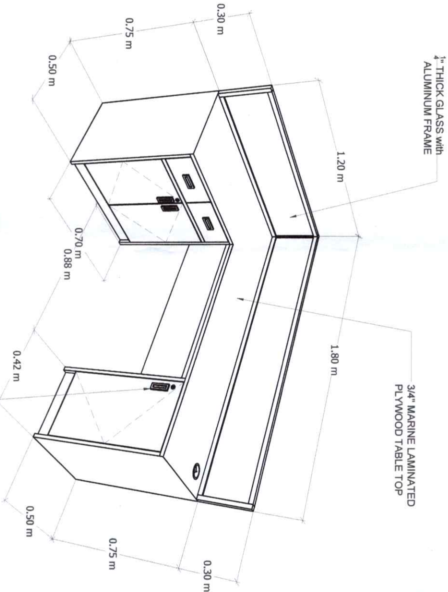
EXTERIOR PARTITION ISOMETRIC DRAWING
